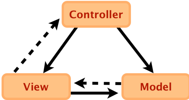
Figure 3.1: Model-View-Controller concept
